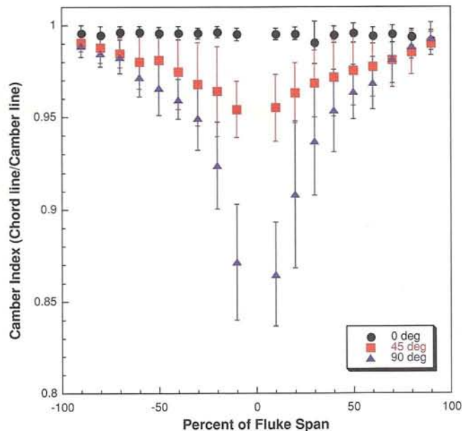
Figure 5. Mean values of camber index ( \pm SD) as a function of percent of fluke span for different experimental deflections (0°, 45°, 90°). The central axis of the tail is 0% and the fluke tip is 100%. Sections from the right fluke are indicated by negative span values and the left fluke with positive span values.
